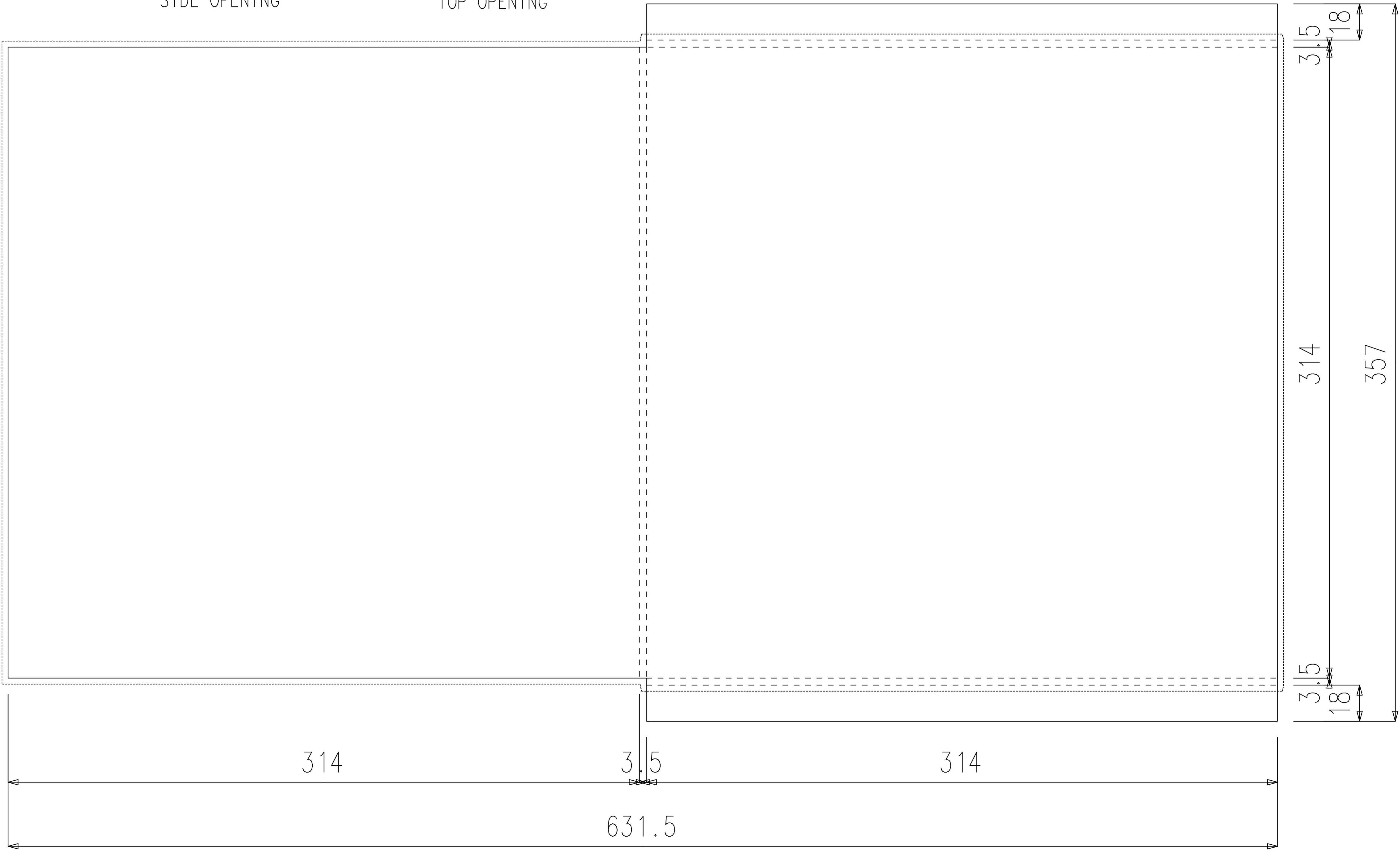
SIDE OPENING
